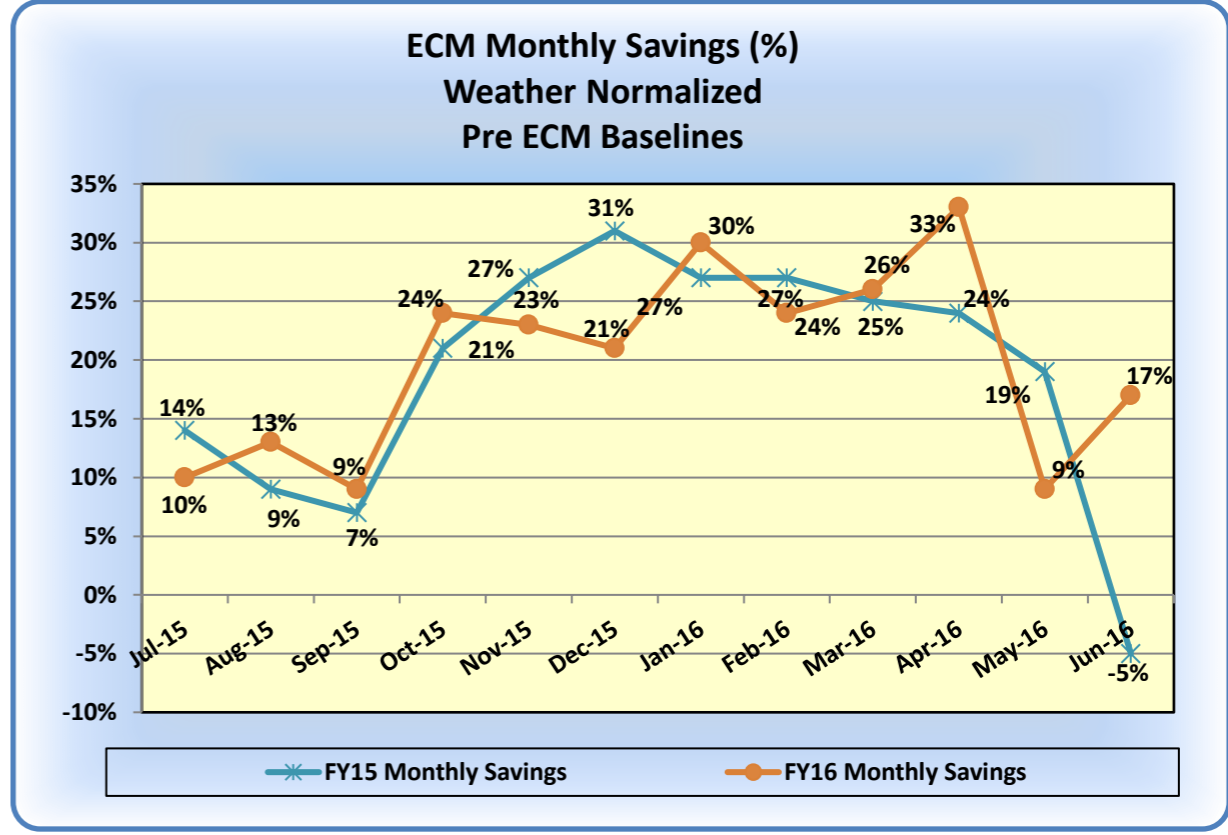
Monthly savings increased from -5% to 17% compared to last year with tuning the buildings added to ECMs.
