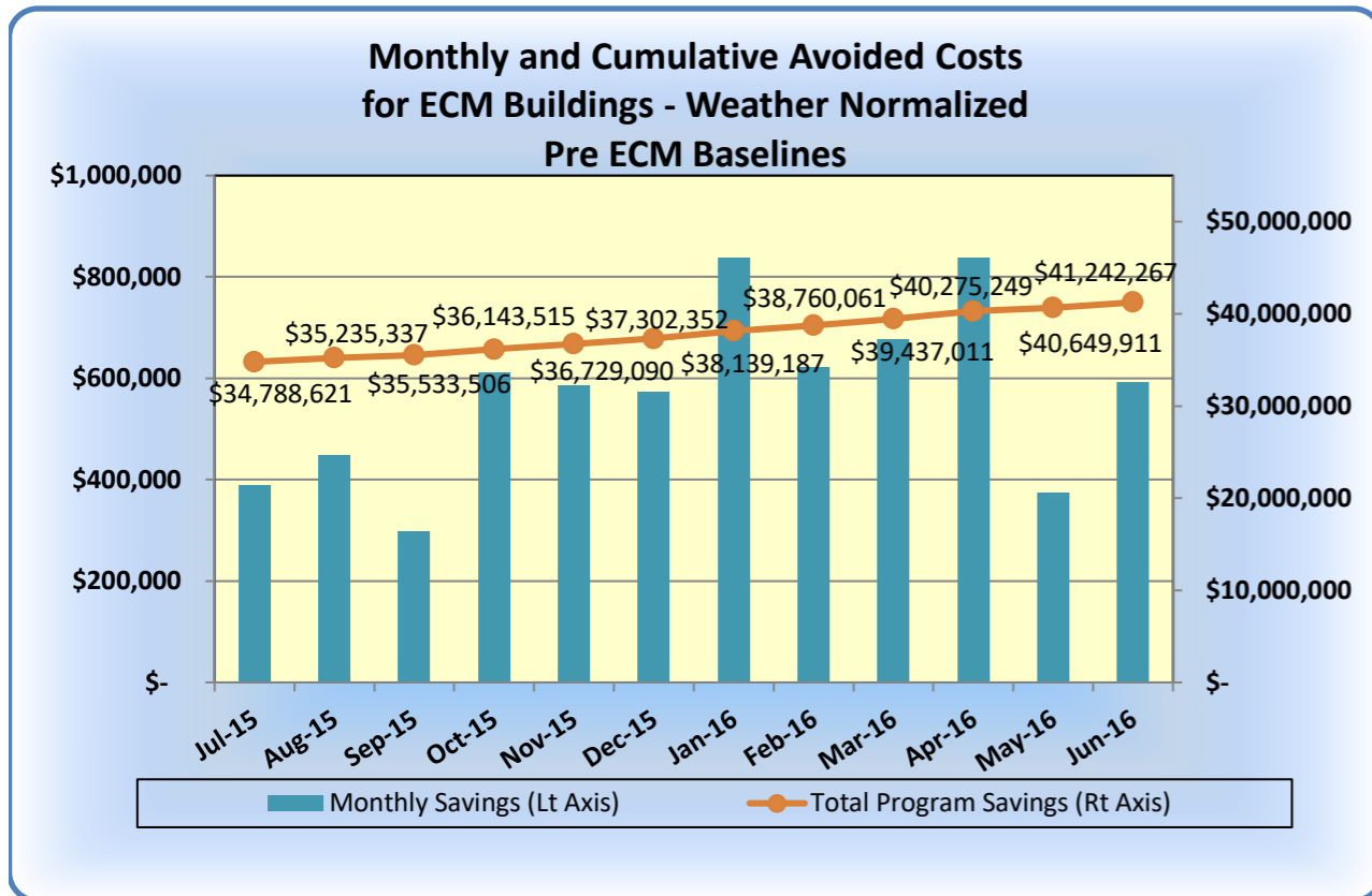
Graph1: Monthly savings increased for the buildings where we have tuned the HVAC systems to $592,051. This results in a total program savings of $41M.
